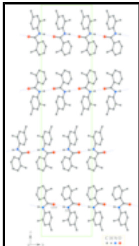
Fig. 2. Crystal structure of the title compound viewed in the bc -plane. Chains running along the b axis generated by N—H···O# hydrogen bonds are shown by dashed lines. [Symmetry code (#): -x + 1/2, y - 1/2, z ]. H atoms not involved in hydrogen bonding have been omitted.
